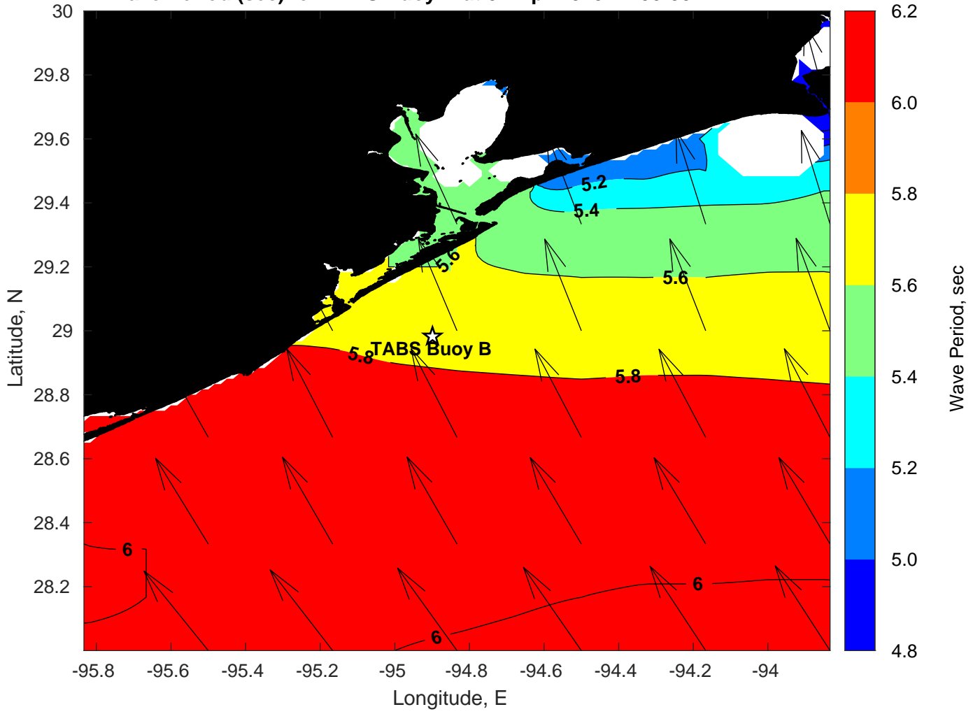
Wave Period (sec) for TABS Buoy B at 04-Apr-2023 12:00:00
